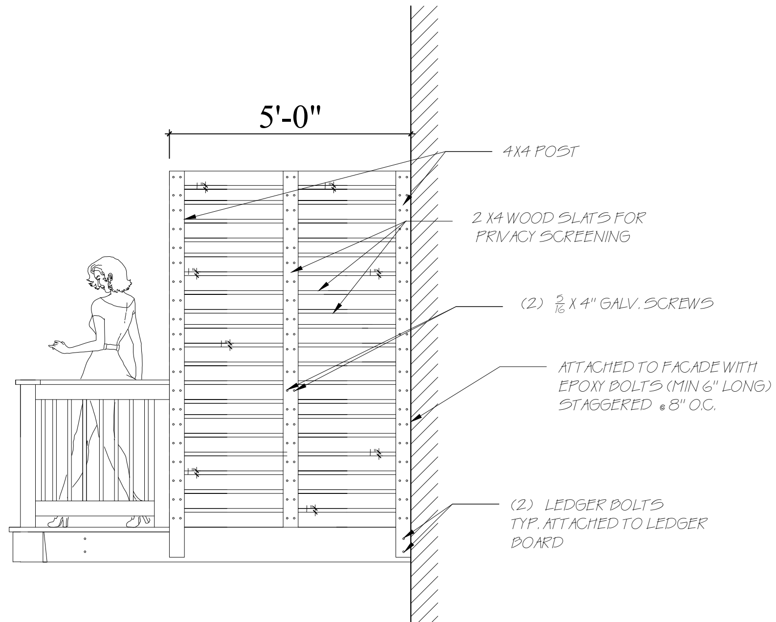
① VIEW FROM NEIGHBOURS SIDE SCALE: 1/2"=1'-0"
